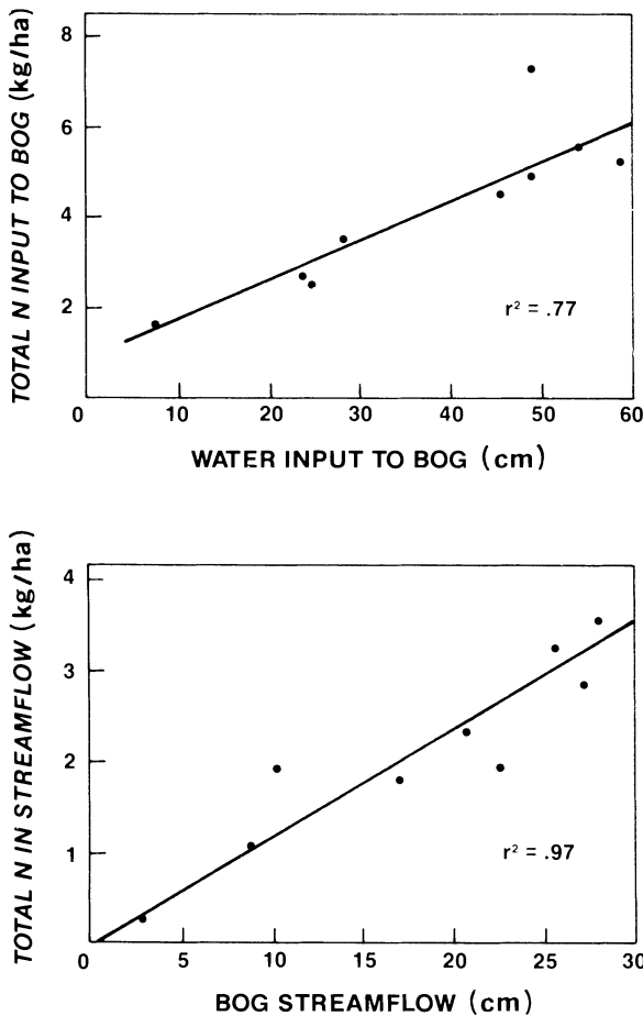
FIG. 3. Seasonal total N input and output in relation to the amount of water carrying it.
