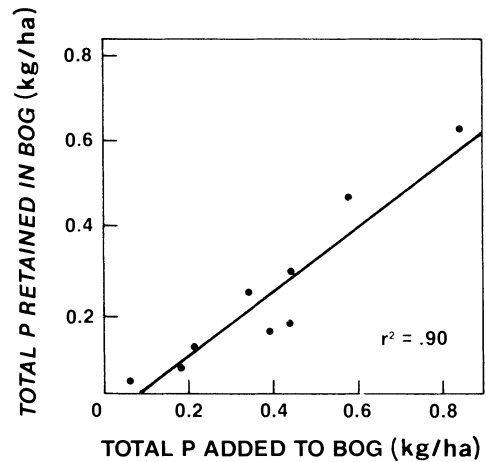
FIG. 4. Seasonal total P added to and retained by the bog.
