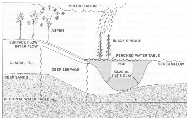
FIG. 2. Cross section of Watershed Number 2 showing water flow routes.
